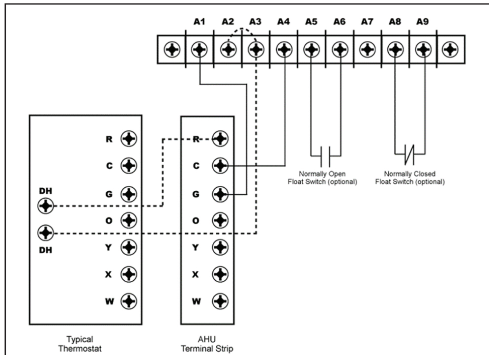
FIGURE 3: WIRING DIAGRAM
