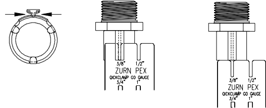
Gauging Area
