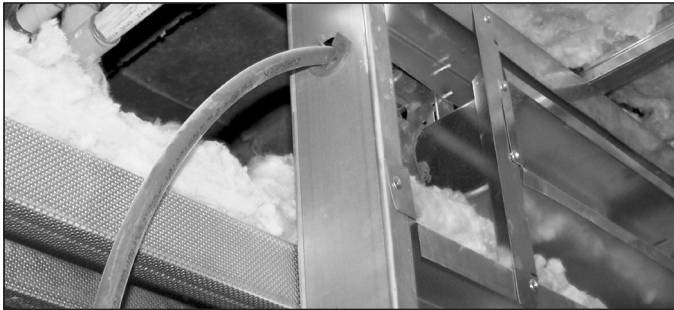
Zurn PEX tubing sleeved through steel stud for protection.
