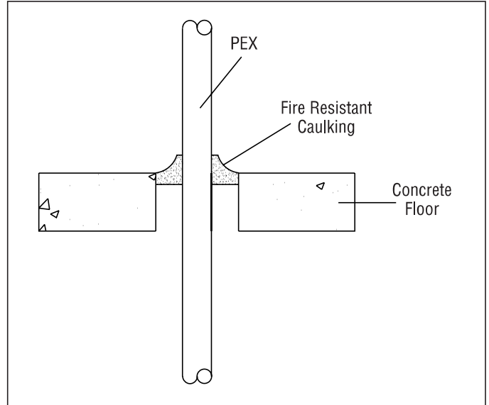
Fire Resistant Caulking Through Floor
