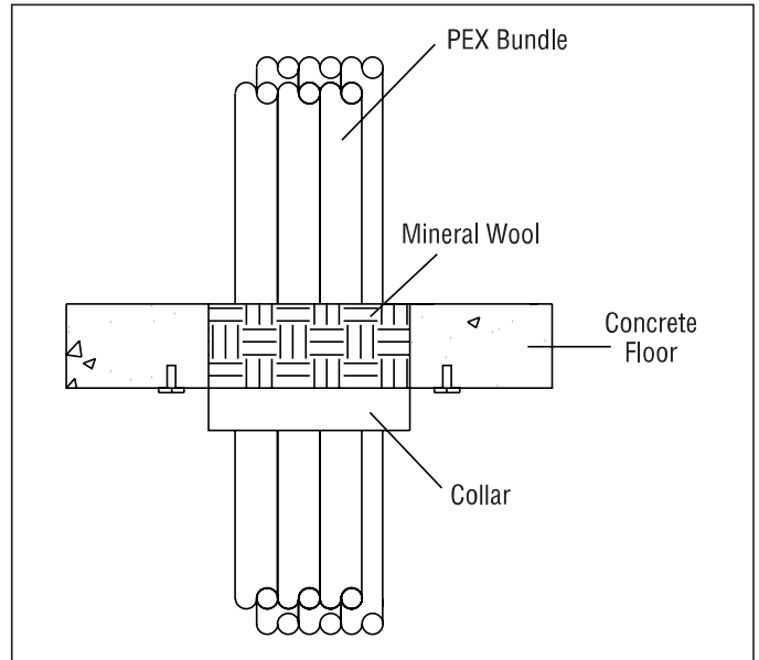
PEX Bundle Through Floor
