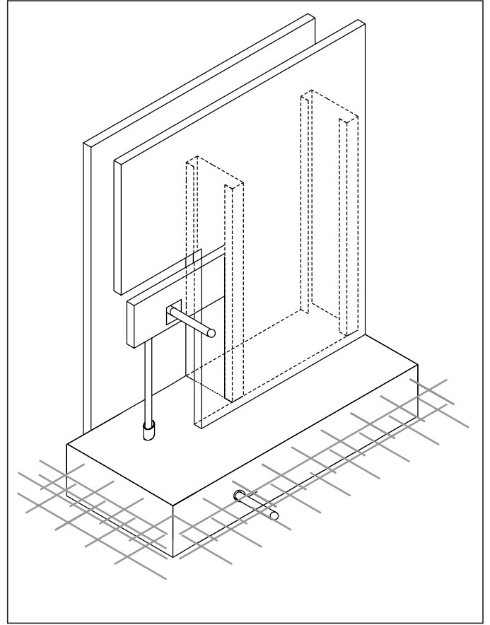
Example of Fixture Supply in Commercial Construction
