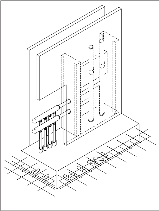
Example of Copper Manifold (QCM43-_GX) in Commercial Construction
