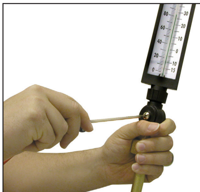
Loosen single screw (A).
