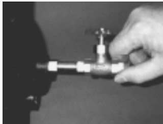
Step 6: Connect the valve/nipple assembly from step 5 to the Series 717R main valve at the downstream port as shown.
