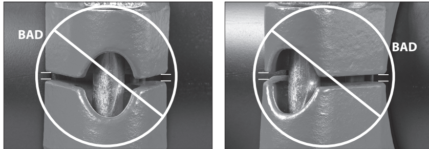
IMPROPERLY ASSEMBLED JOINT – BOLT PAD GAP/UNDER-TIGHTENED
