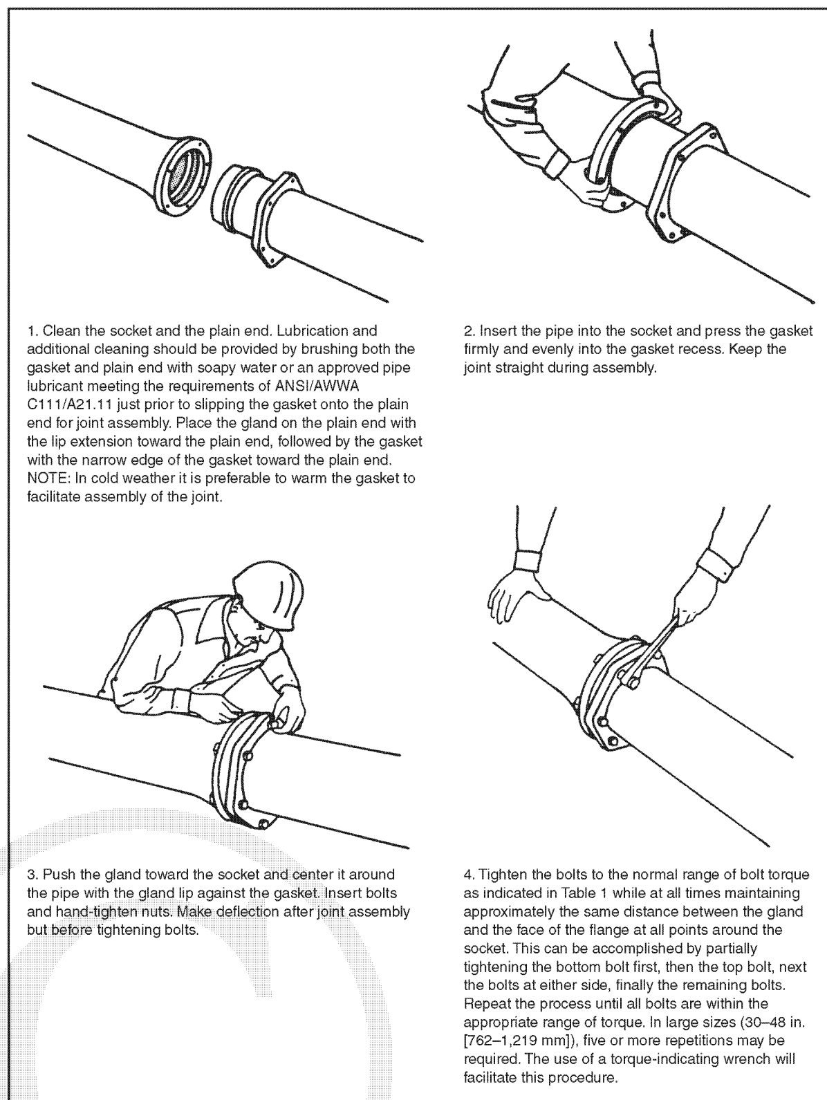
Figure 3 Mechanical-joint assembly
