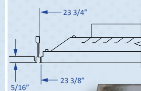
1400FL Fine Line / Narrow-T 1444RG-FL
