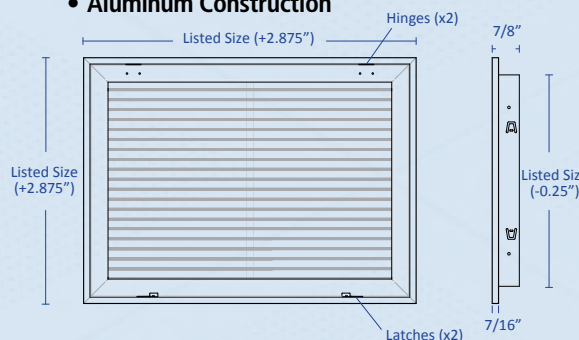
Model 290 Shown Open
