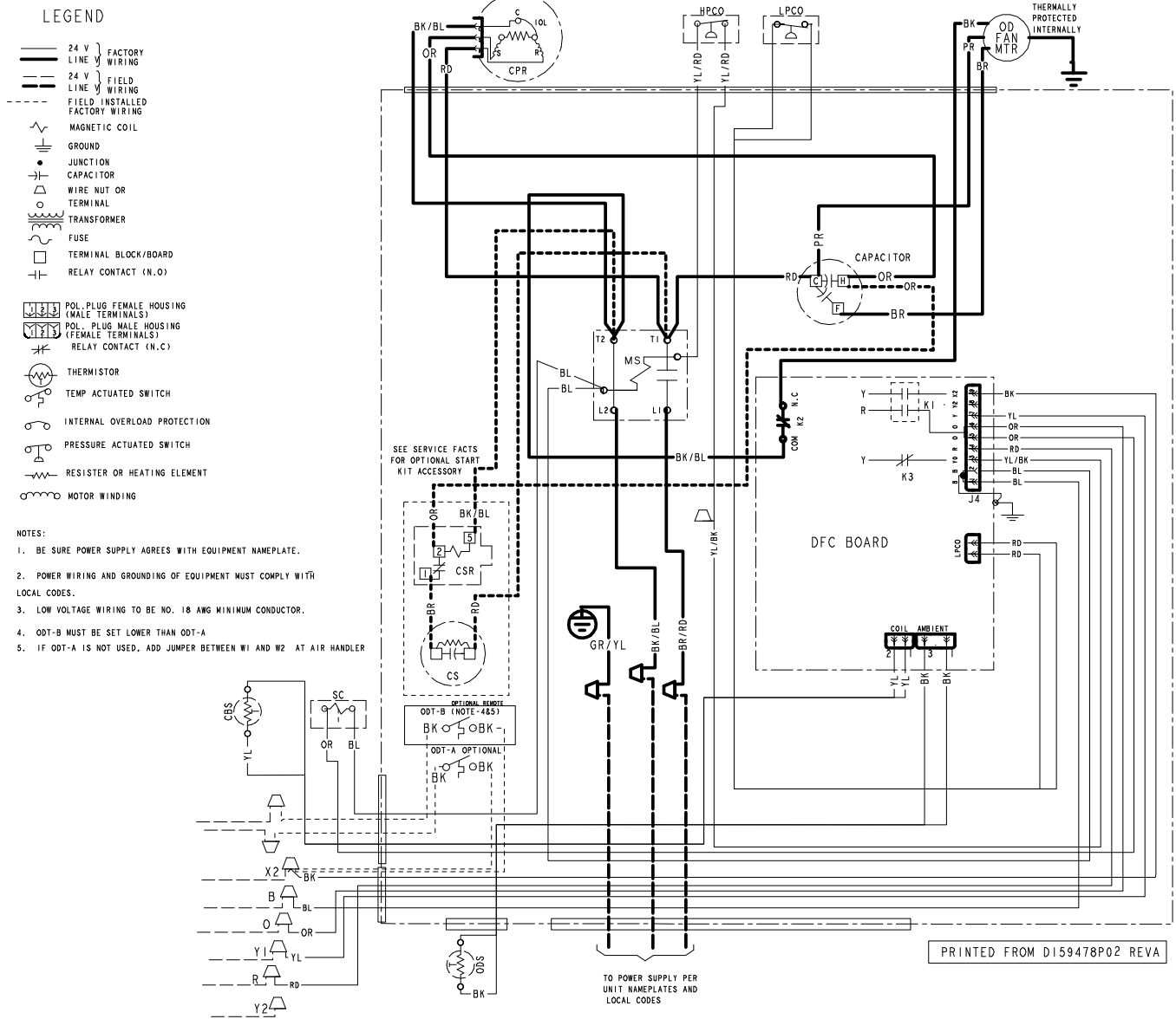
Figure 2. 1.5, 2.0, 2.5 & 3.5 Ton Models
