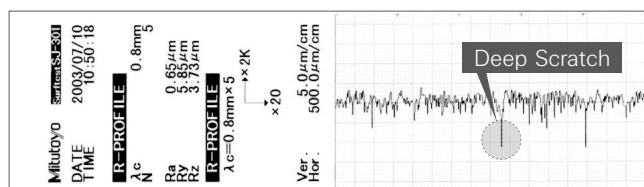
After Sanding with Paper Disc
