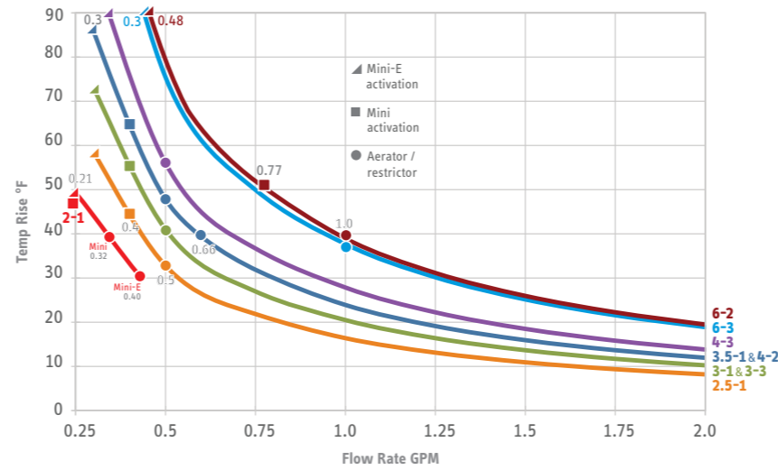
1.8 – 5.7 kW Mini./Mini-E Temperature Rise vs. Flow Rate at Max Rated Voltage
