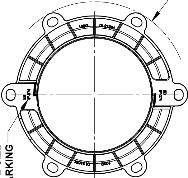
2"-12" FLANGE DETAIL
