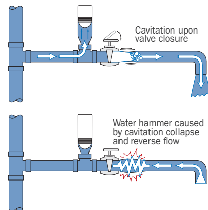
Fig 2: Shut-off valve in MIDDLE of long pipe run
