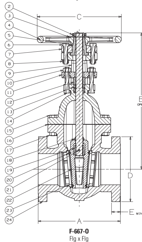
F-667-0 Flanged
