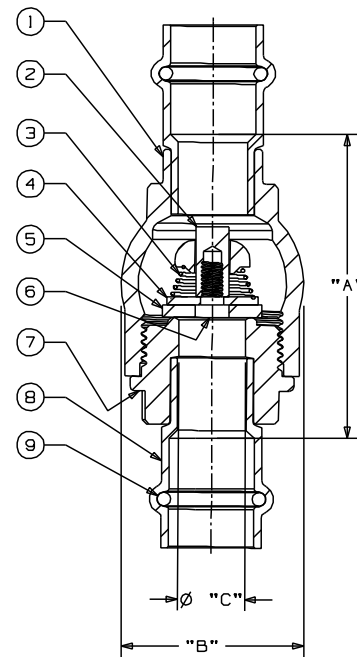
PF480-Y (PTFE Disc) P x P
