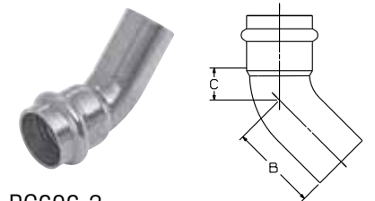
PC606-2 45° Elbow Ftg x P – Wrot
