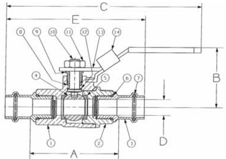
PC585-70-LL P x P
