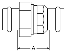
PC733-4 Union P x M – Brass Rod
