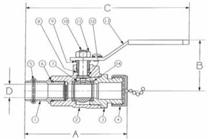
PC585-70-66-HC P x Hose
