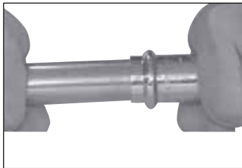
Figure 6 — Inserting the tube to proper depth
