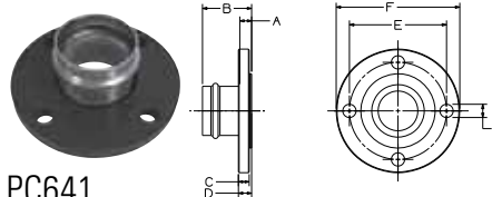
PC641 Companion Flange P x Flange - Wrot
