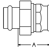
PC733-3 Union P x F – Brass Rod
