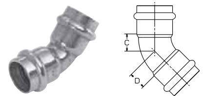
PC606 45° Elbow P x P – Wrot
