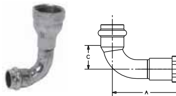
PC607-3 90° Elbow P x F - Wrot
