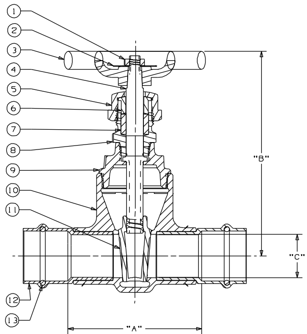
PF113 P x P
