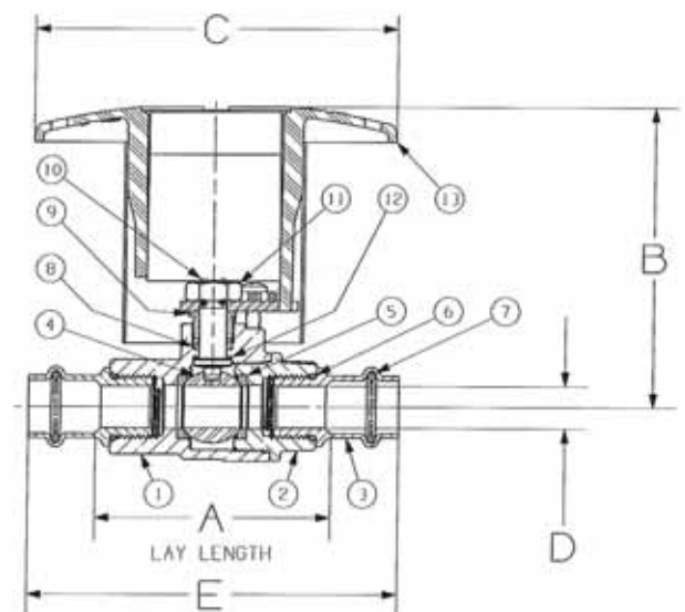
PC585-70-NS P x P
