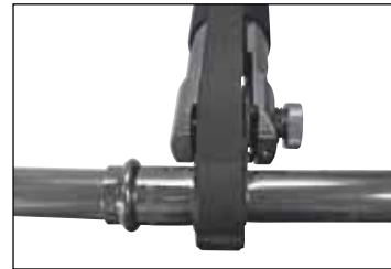
Figure 8 — Jaw set should be square to tubing
