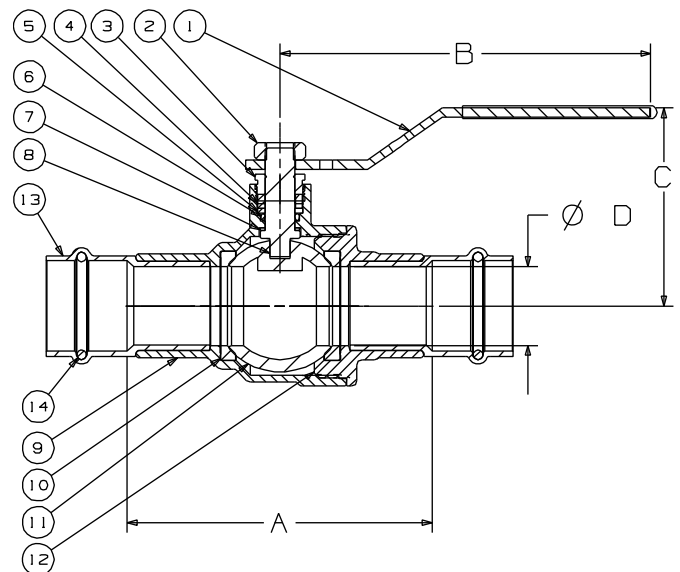
PFFP60 P x P
