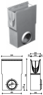
FILCOTEN Pro Sump Unit 200
