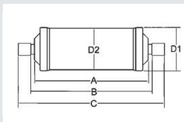
Solder Connection
