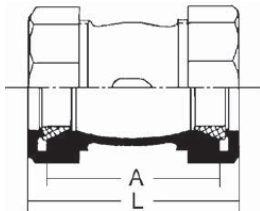
440T Coupling - Short
