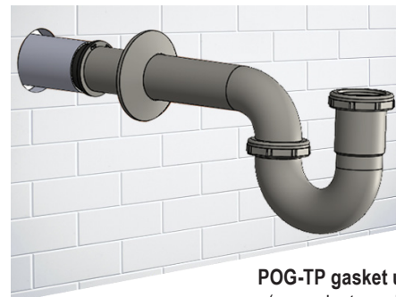
POG-TP gasket used (no sealant needed)
