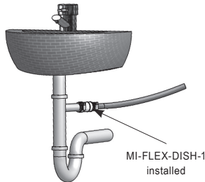
(Typical Installation underneath a sink)
