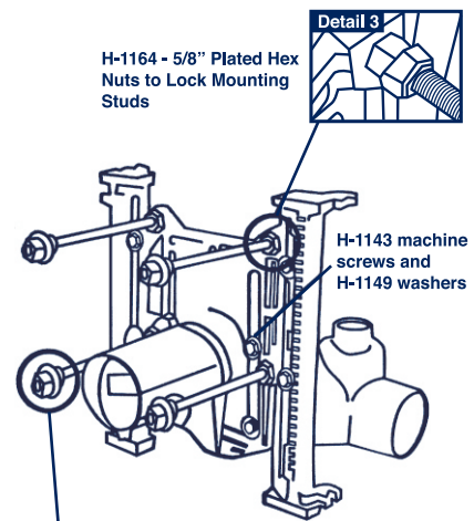
MC-10-PFH Finishing Hardware (Cap Nuts & HDPE Washers including Bowl Saver Washer)
