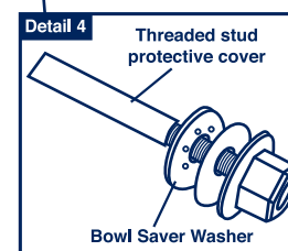
MC-10-PFH Finishing Hardware (Cap Nuts & HDPE Washers including Bowl Saver Washer)
