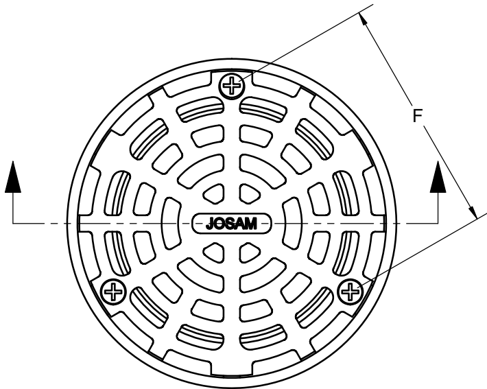
5A-6A-7A-8A SLOT WIDTH : 1/4" MEETS ADA AND HEEL-PROOF REQS.
