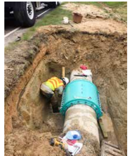
JCM 114 Mechanical Joint Bell Repair Sleeve installed over problematic leaking Asbestos Cement Coupling
