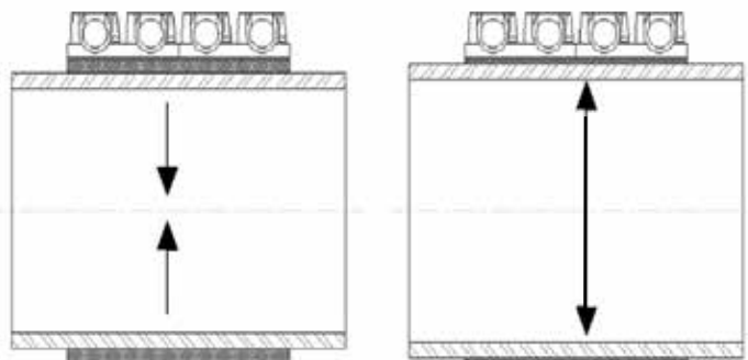
As pipe contracts, gasket expands and releases stored energy.
