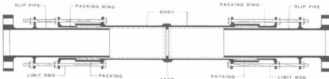
JCM 802 Double End Expansion Joint
