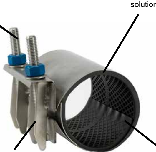
Image Reflects 7" Clamp Width
