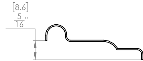
CROSS SECTION A-A SCALE 1 : 1
