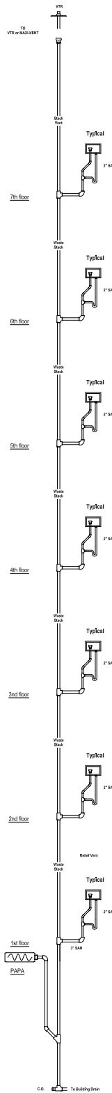
“Studor Single Pipe System (SSPS)”
