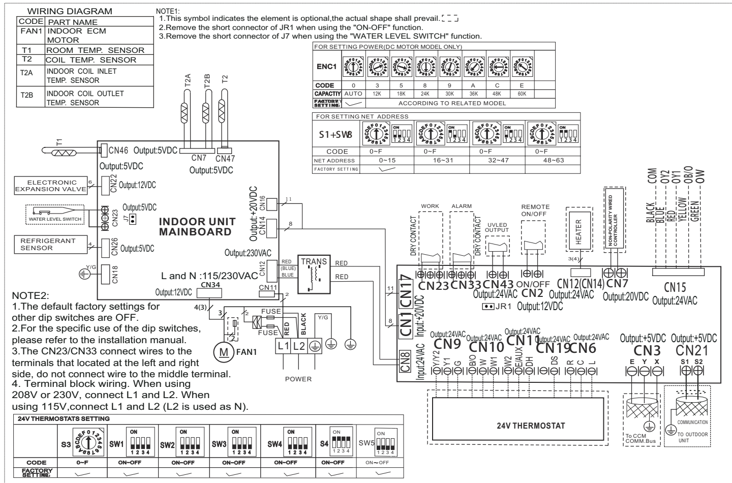
Fig. 13 —Wiring Diagram Sizes 30K, 36K, 48K, 60K
