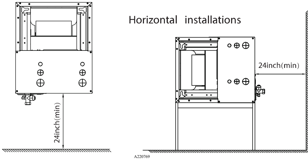
Fig. 7 — Clearances
