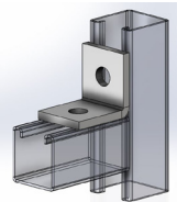
FIG. 9022CA 2-hole corner angle 1-7/8 x 2
