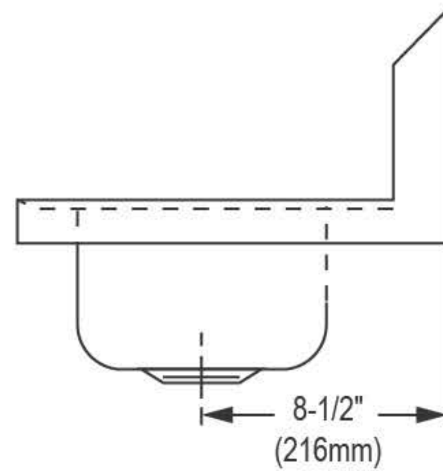
SECTION THROUGH RIM
