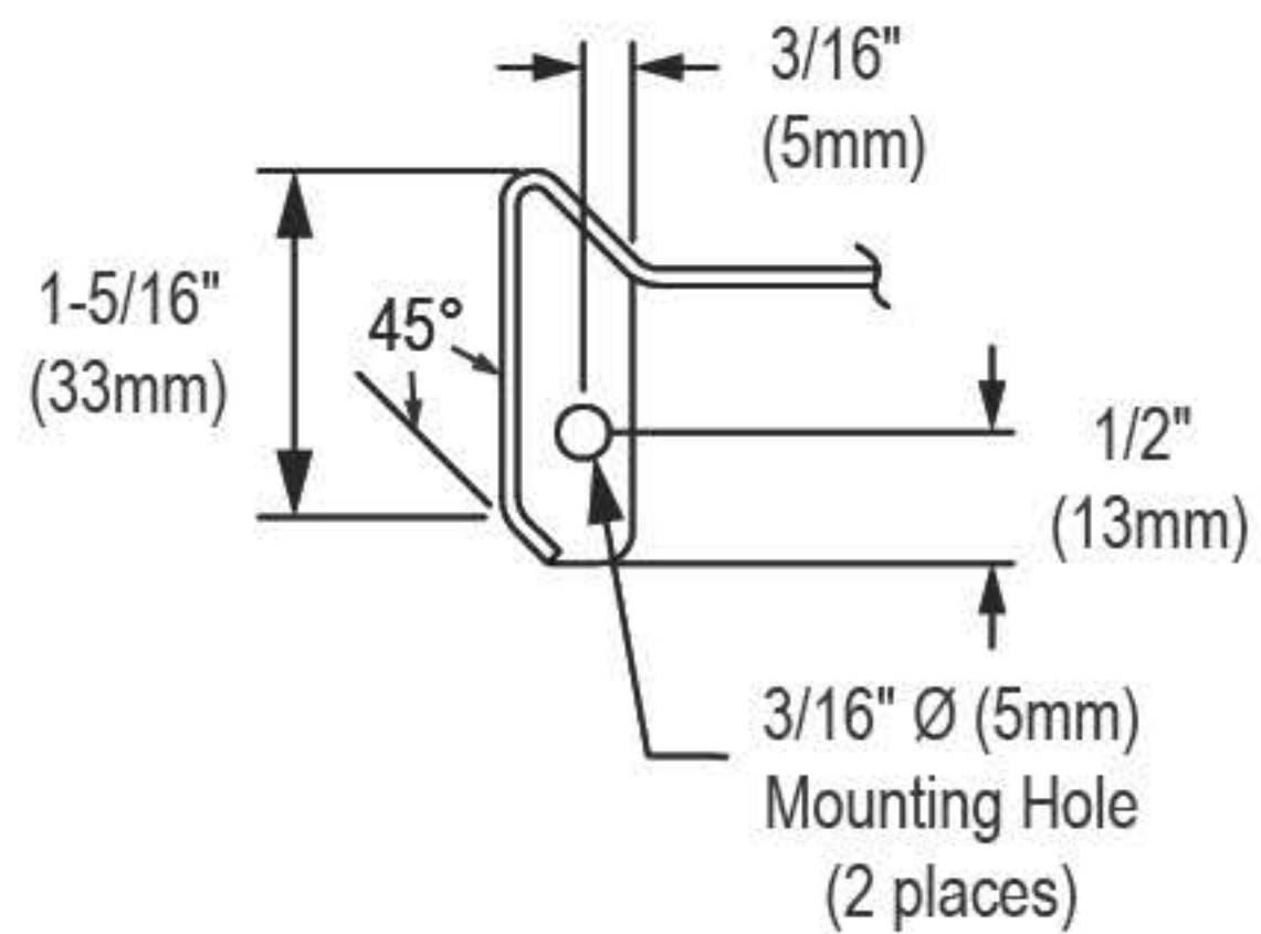
SECTION THROUGH RIM
