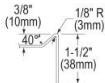
SECTION THROUGH RIM
