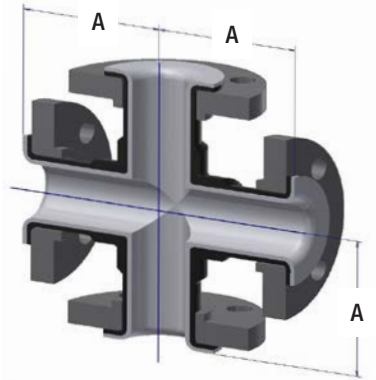
Equal Cross
