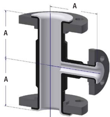
Reducing Tee
