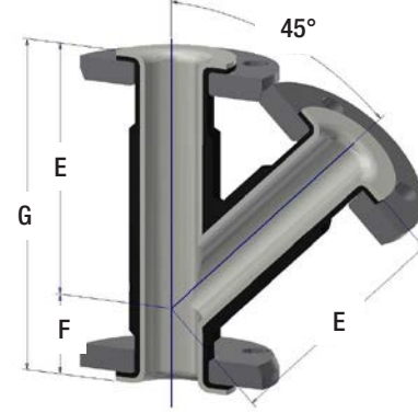
Lateral Half
