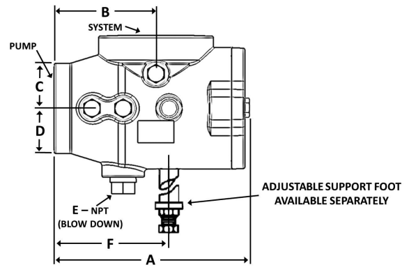
Threaded x Threaded Models
