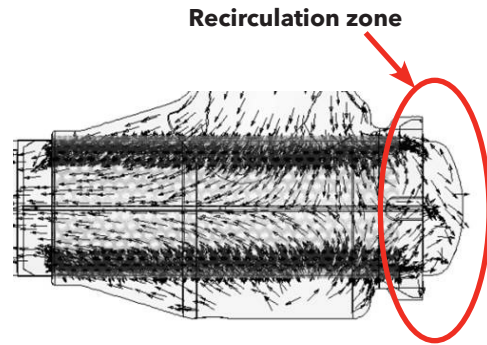
Figure 1 Velocity vectors in current designs
