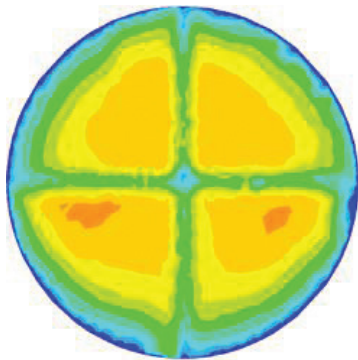
Figure 3 Flow uniformity at pump suction from current designs
