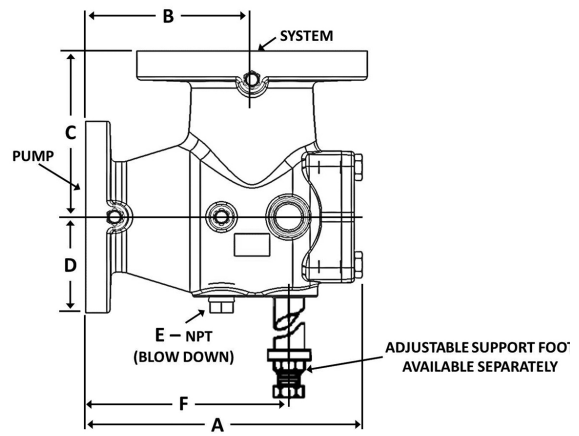
Flange x Flange Models
