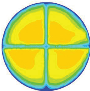
Figure 4 Flow uniformity at pump suction from new design
