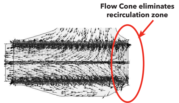
Figure 2 Velocity vectors in new Bell & Gossett design
