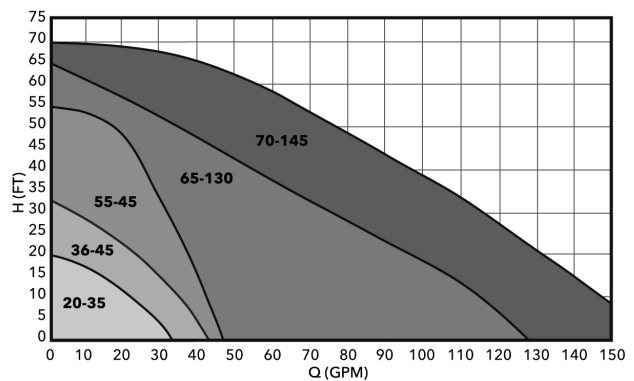
ecocirc XL High Head Performance Range
