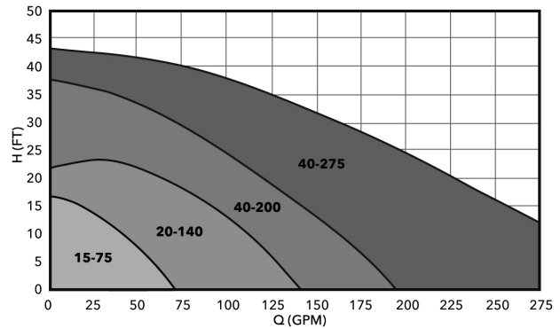
ecocirc XL High Flow Performance Range
