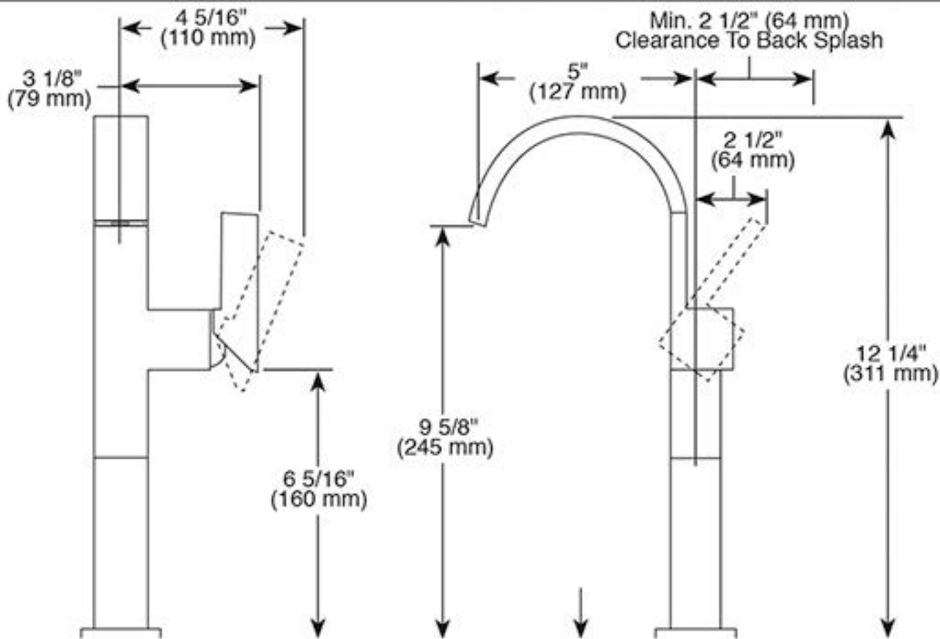
RP72411 ▲ Grid Strainer Drain less overflow holes
