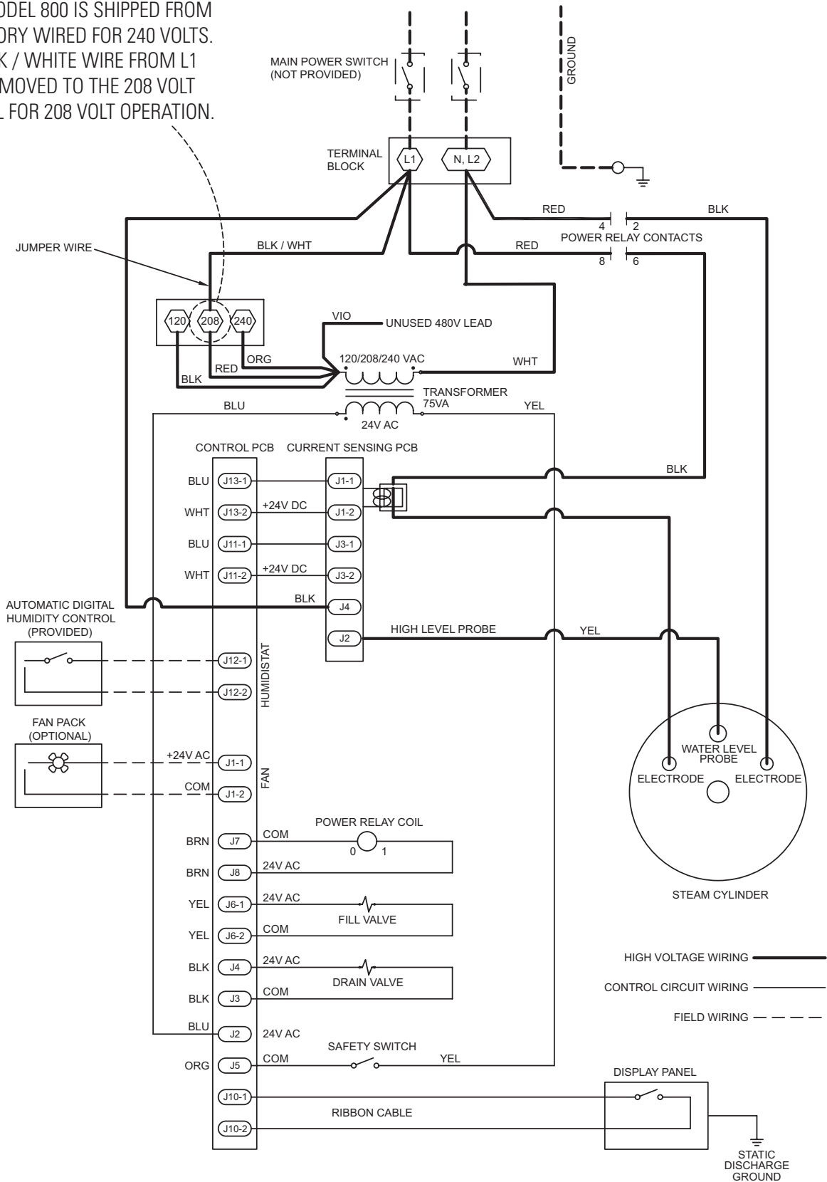
FIGURE 9 – 208 VAC Wiring Diagram
