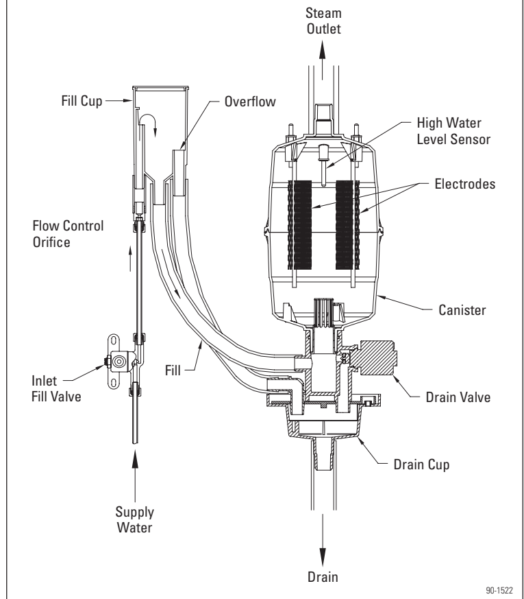
FIGURE 1 – Fill and Drain System and Canister
