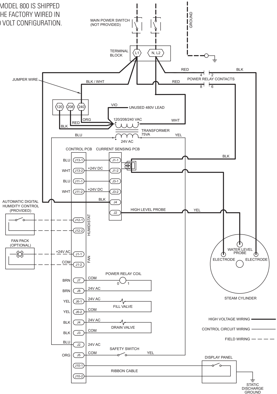
FIGURE 8 – 240 VAC Wiring Diagram
