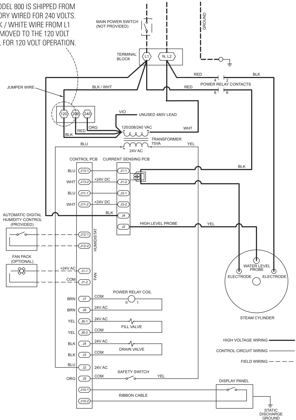
FIGURE 10 – 120 VAC Wiring Diagram
