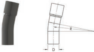
1 1/4° Bell End
