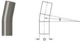
1 1/4° Plain End
