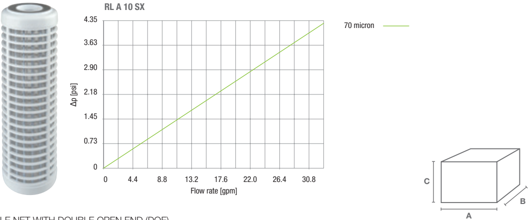
RL A SX | STAINLESS STEEL AISI 316 WASHABLE NET WITH DOUBLE OPEN END (DOE)
