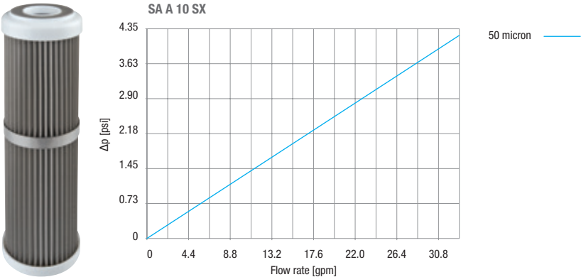
FLOW RATE vs PRESSURE DROP Δp | - Testing mode: 68°F - 43.5 psi (20°C - 3 bar)
