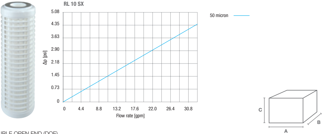
RL SX | POLYESTER WASHABLE NET WITH DOUBLE OPEN END (DOE)
