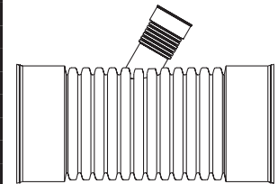
60° REDUCING WYE N-12 ST AND N-12 WT
