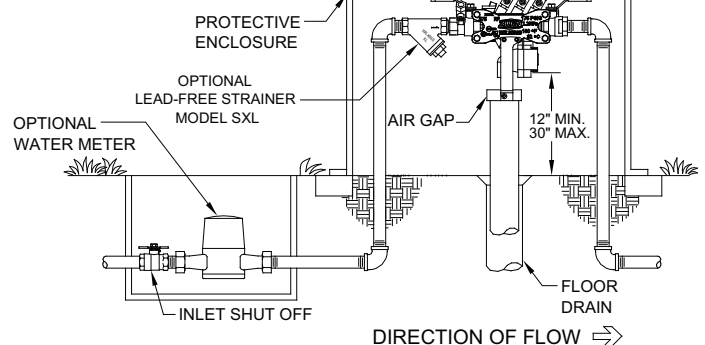
OUTDOOR INSTALLATION
