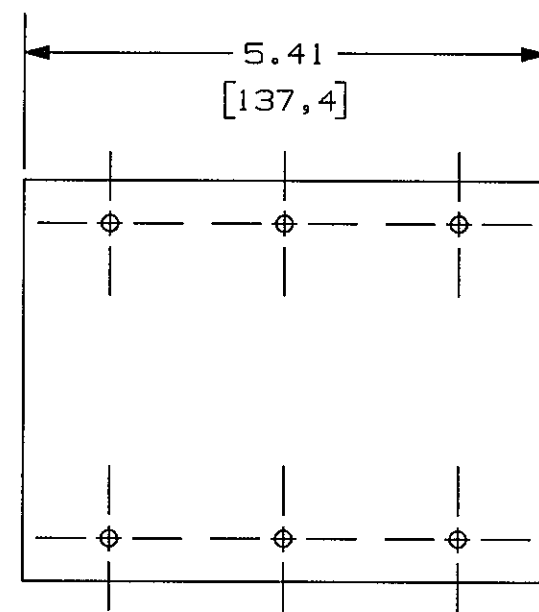
CATALOG NUMBER S1R8CSPG 1-G 1.6" OPENING
