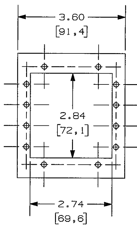
CATALOG NUMBER S1R8CSPA 2-GANG (4) EXTRON AXP
