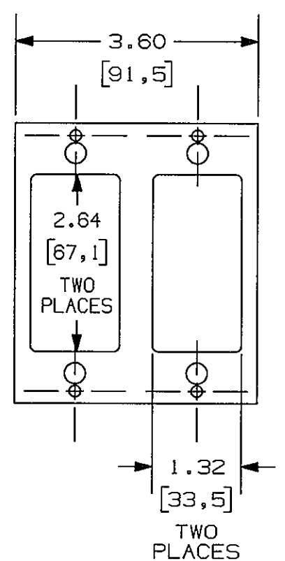
CATALOG NUMBER S1R8CSPM 2-G STYLIN
