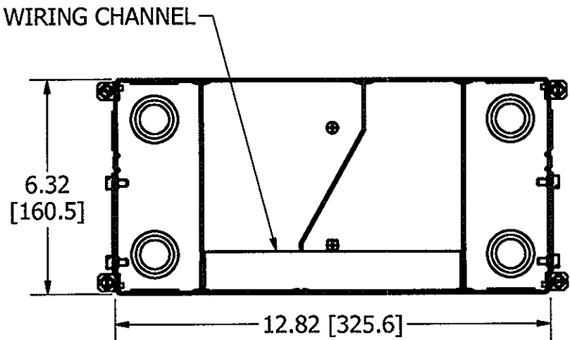
SECTION A-A VIEW THROUGH BOX BELOW TRANSITION
