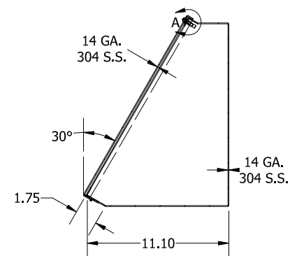
SECTION A-A VIEW (INSIDE LEFT OF ENCL.)
