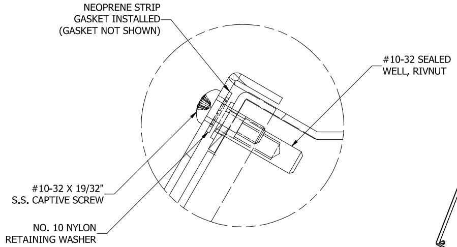
DETAIL A (3 PL.) (LID ATTACHMENT DETAIL)
