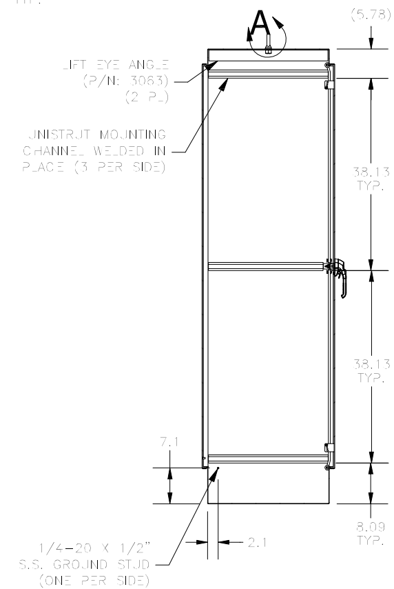
SECTION A-A (INSIDE SIDE OF ENCL.) (TYP.)
