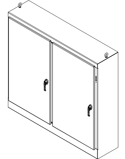
REMOVABLE MULLION WITH DISCONNECT LATCH CATCH ASSEMBLY (SEE HWDHFW500003 FOR DETAILS)
