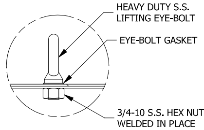
DETAIL A (2 PL.) (LIFT-EYE DETAIL)
