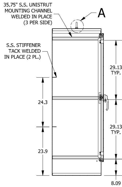
SECTION A-A (INSIDE RIGHT VIEW OF ENCL.)
