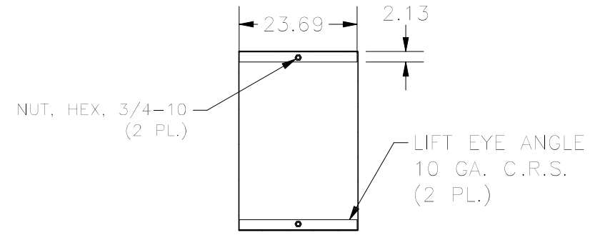
SECTION C-C (INSIDE VIEW OF ENCLOSURE)
