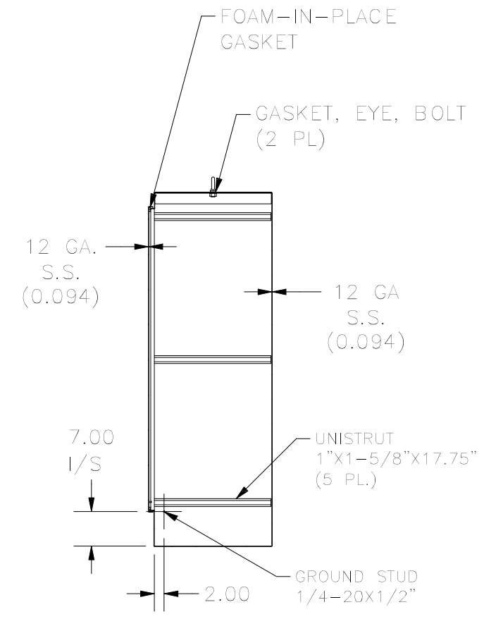
SECTION B-B (INSIDE LEFT VIEW OF ENCLOSURE)
