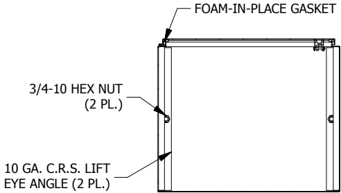
SECTION C-C (INSIDE TOP OF ENCL.)
