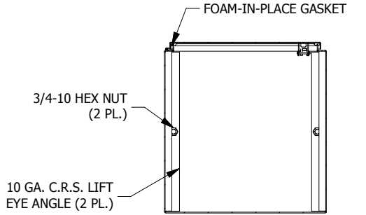
SECTION C-C (INSIDE TOP OF ENCL.)
