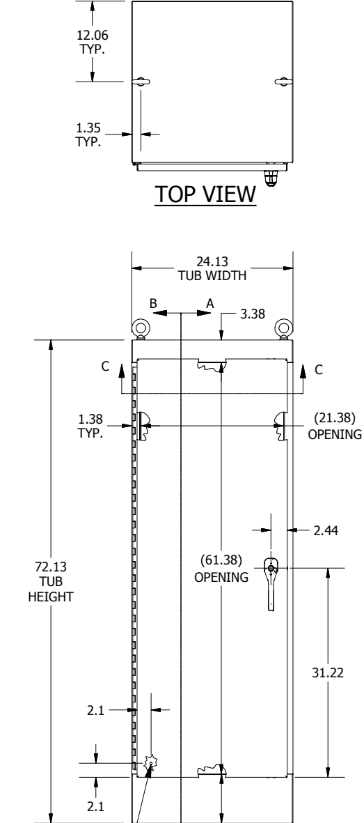
FRONT VIEW
