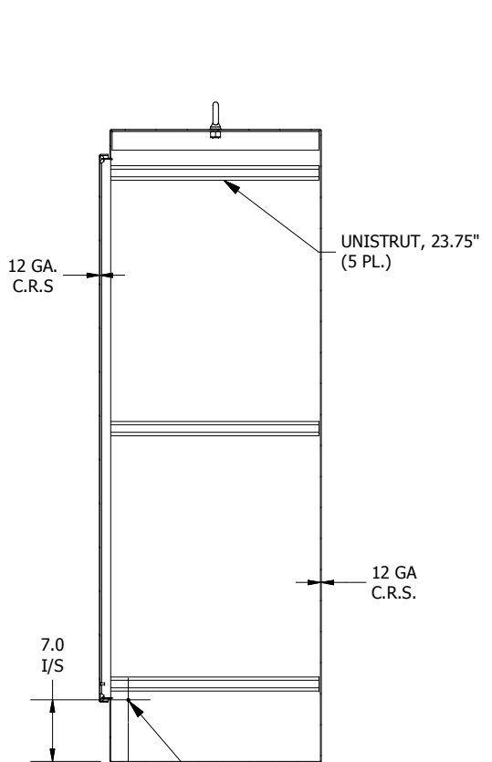
SECTION B-B (INSIDE LEFT OF ENCL.)
