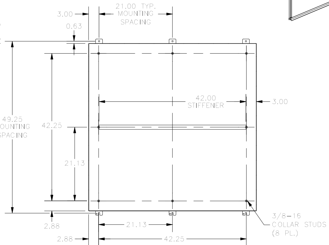
SECTION A-A (INSIDE BACK VIEW OF ENCL.)
