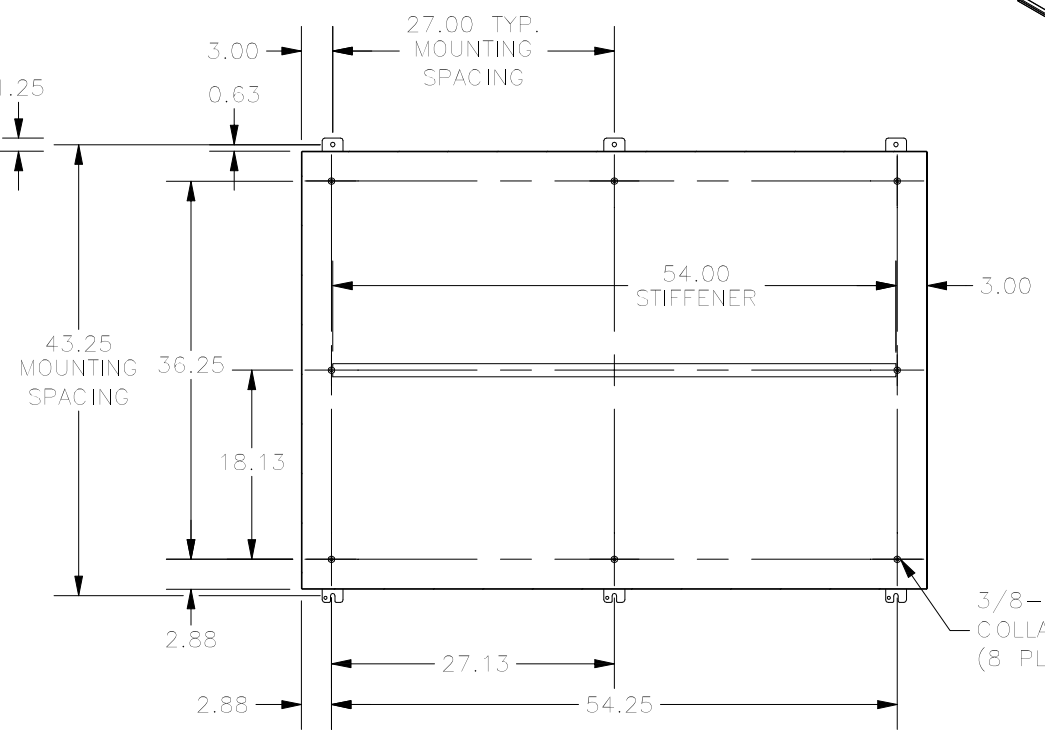
SECTION A-A (INSIDE BACK VIEW OF ENCL.)
