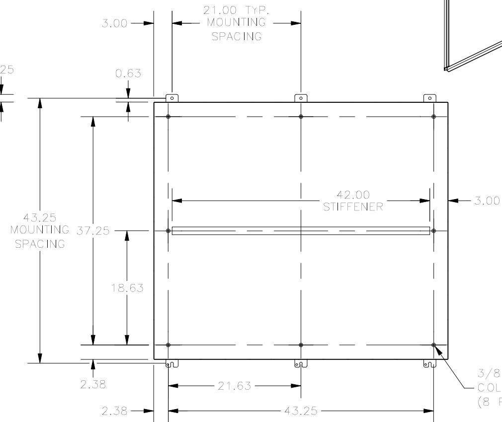
SECTION A-A (INSIDE BACK VIEW OF ENCL.)
